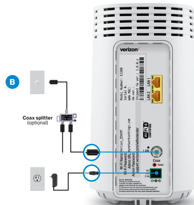
Setup Diagram
